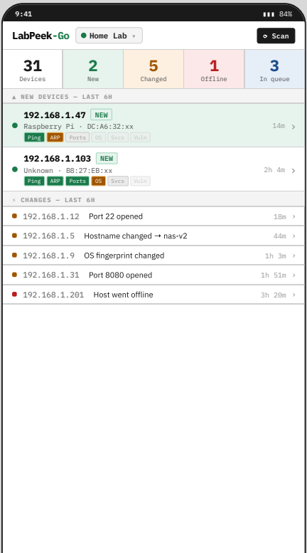
V1 · Light — KPI cards + alert lists
